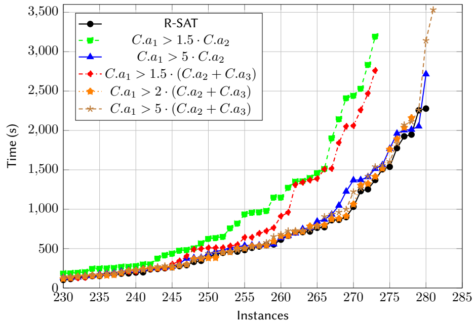
Figure 12: Cut-off value comparison for relative size criterion on the DEC-LIN Track.
